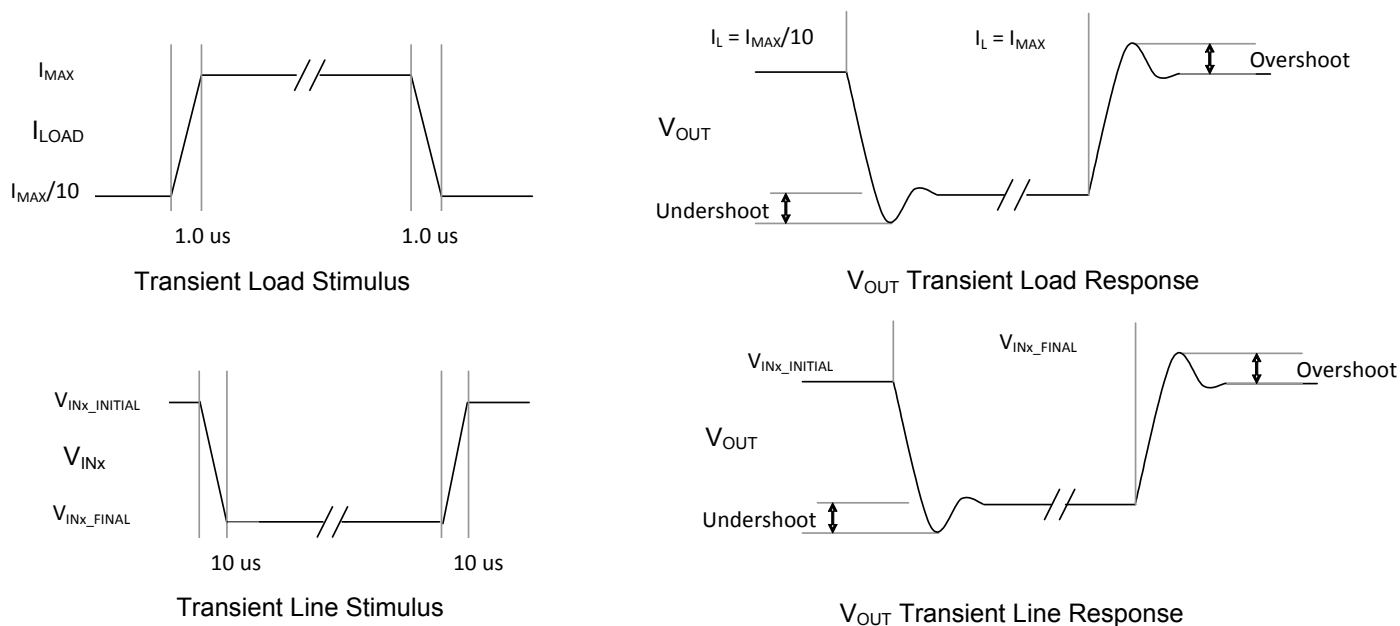
Figure 31. Transient Waveforms
