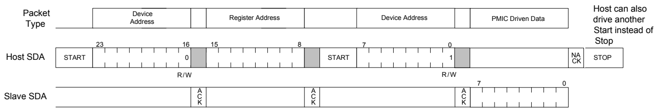
Figure 34. I²C Read Example
