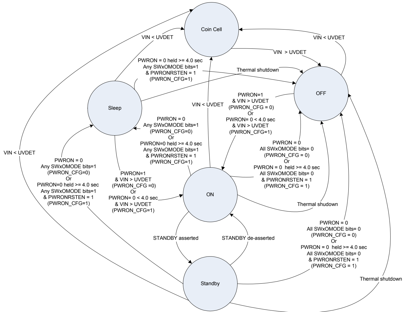
Figure 8. State Diagram
